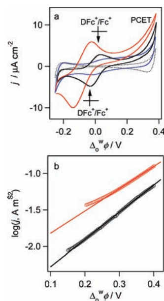
Figure 5. (a) Cyclic voltammetry at a water–DCE interface obtained with the cell illustrated in Scheme 3 in the presence of 50 μM CoP and different electron donors ( x = 50 and y = 5 ): Fc (black), DFc (red), and FcCA (blue). The dotted curve represents the background catalytic CV ( x = 0 and y = 0 ). (b) Tafel plots the background-subtracted catalytic current in the forward scan for Fc (black) and DFc (red).
