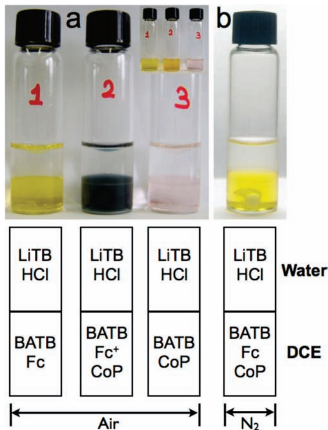
Figure 2. (a) Photographic illustrations of two-phase reactions controlled by \text{TB}^- partition after shaking a couple of seconds: the top aqueous phase containing 5 mM LiTB + 10 mM HCl was the same for all three flasks; the bottom DCE phase contained 5 mM Fc, 5 mM \text{Fc}^+ + 50 \mu\text{M} CoP, and 50 \mu\text{M} CoP in flask 1, 2, and 3, respectively; the inset shows the flasks before adding the top aqueous solution. (b) Two-phase reaction under anaerobic conditions with other conditions the same as flask 2 in Figure 2a. The notations under the figure illustrate the solution composition of each flask.
