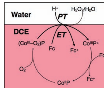
Scheme 4. Interfacial PCET Mechanism
